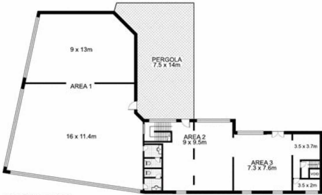
GROUND LEVEL
